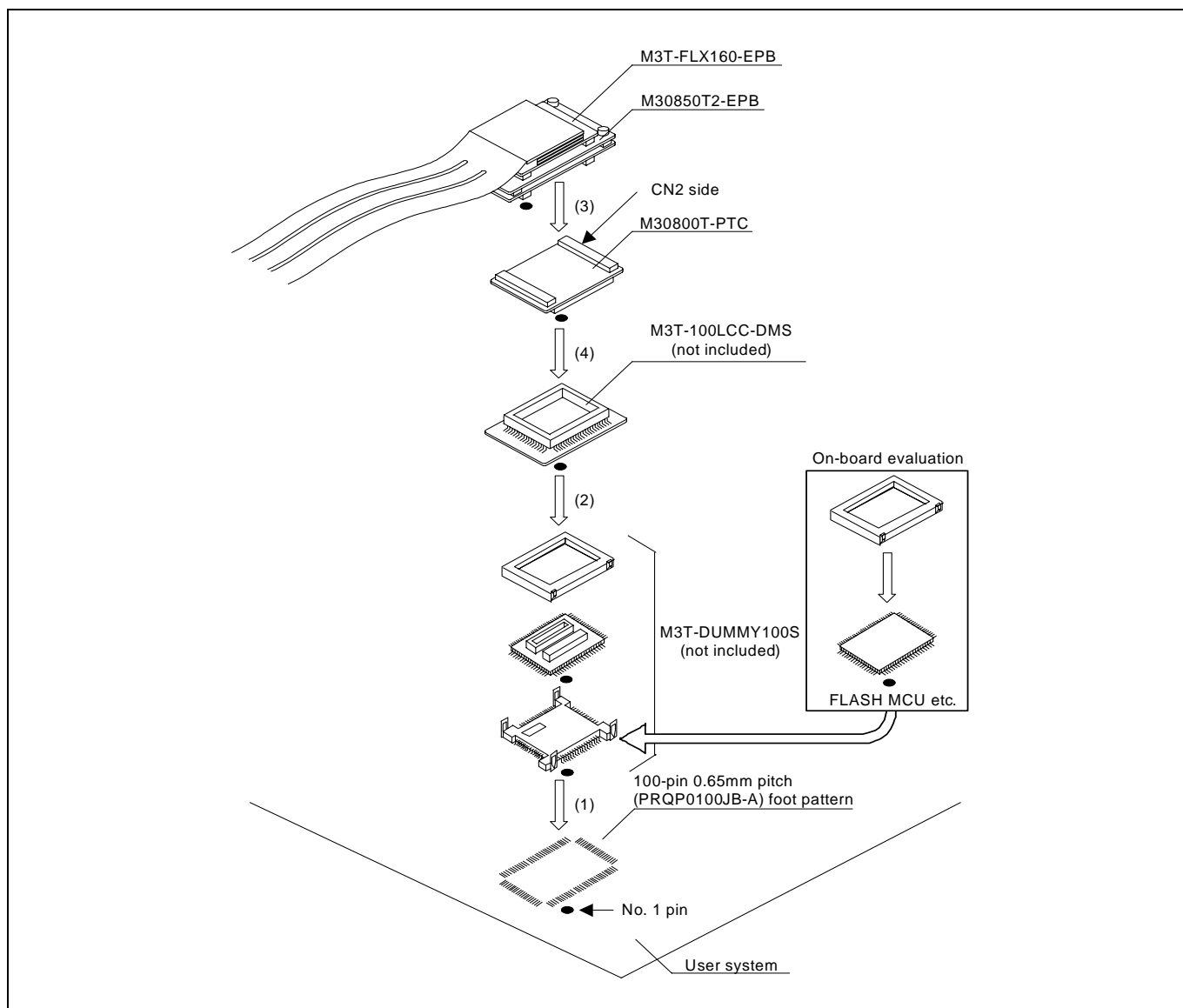
Figure 2.11 Connecting to a 100-pin 0.65mm pitch foot pattern (3/3)
